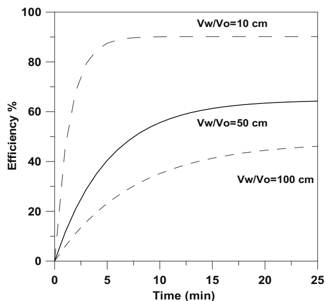
Figure 7 Concentration profiles: effect of change in the ratio of the volume of the two phases.
